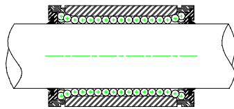
Recirculating rolling ball element bearings that require seals and metal-to-metal contact with the shaft and raceways
